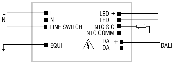
Diagram for 40W - Collegamento per 40W
